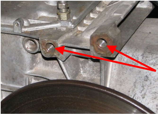
Photo 3: Shows the attachment points for the brake caliper bolts on the right side of the gearbox. The caliper bolts hold the thin metal shim and the brake calipers in place.
