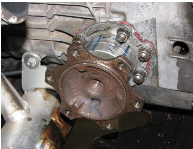
Photo 4: Ladies and gentlemen. Please take your seats. After the CV-joint plate and brake disc are removed from the output hub drive flange, the output hub is exposed in all its glory! The photo shows the flared drive flange on the output hub with its six bolt attachment points. Note the blue "R" (for the right side). Yes, many 2CV owners never get to see the output hubs because they are highly-reliable, long-lasting components which are mostly hidden from sight by the brake components of the 2CV.
